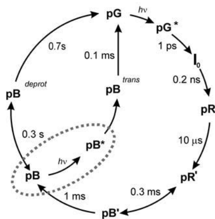
SCHEME 1 Photocycle of PYP. The effect of photon absorption by pB is represented inside the ellipse.
