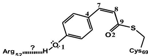
SCHEME 2 The cis -isomer of 4-hydroxycinnamyl thioester in the pB intermediate. The relevant atoms discussed in the text are numbered.
