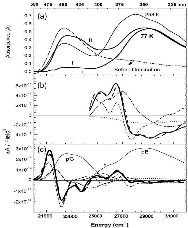
FIGURE 1 (a) Absorption spectra of M100A in glycerol/buffer solution at 298 K: spectra before and after illumination at 450 nm are shown in dotted-dashed and light solid lines, respectively; 77-K spectra (bold solid lines) include I, with mostly pB, and II, a mixture of pG and pB. The field-normalized Stark signal (dark solid line), fit (dark dashed line), and scaled first (light dotted-dashed line) and second (light dashed line) derivatives of the absorption are shown in panel b to spectrum I and in panel c to spectrum II.
